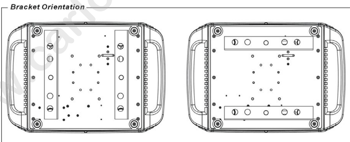
Figure 2-3: Installing Brackets on Luminaire Enclosure
