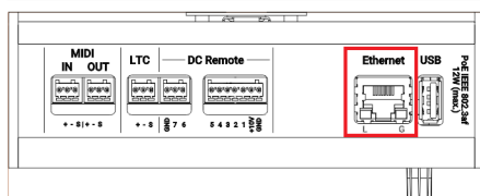
grandMA3 I/O Node DIN-Rail rear panel – Ethernet
