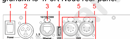
rear panel
