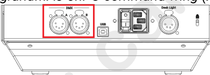
grandMA3 onPC command wing (XT) rear panel – DMX
