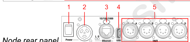
grandMA3 4Port Node rear panel
