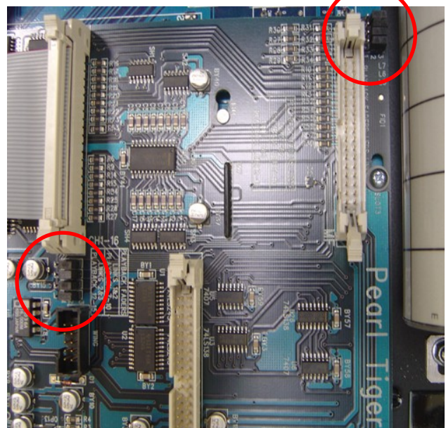
Faders 12-15
